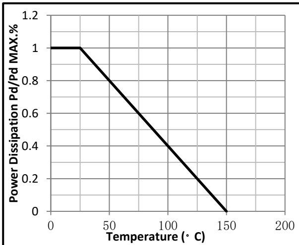
Fig.3 Power Dissipation
